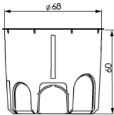
SKETCH
