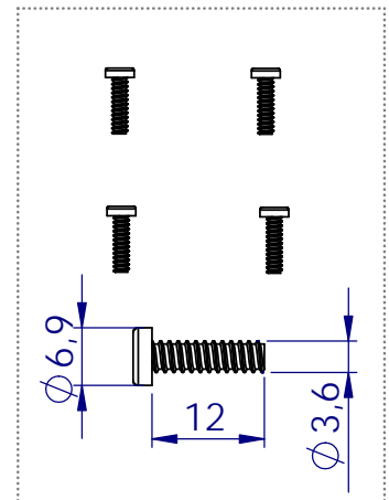
Ref. .T-1316/1 TORNILLOS (4) SCREWS VIS
