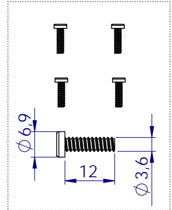
Ref. .T-1316/1 TORNILLOS (4) SCREWS VIS
