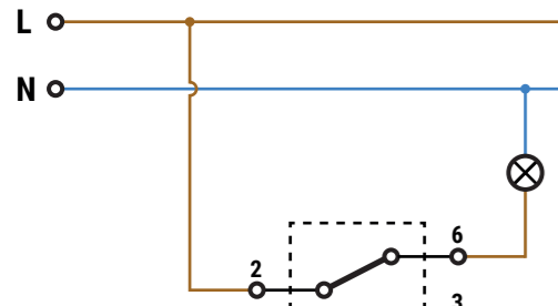
INTERRUPTOR MUR02/MUR02ILU
